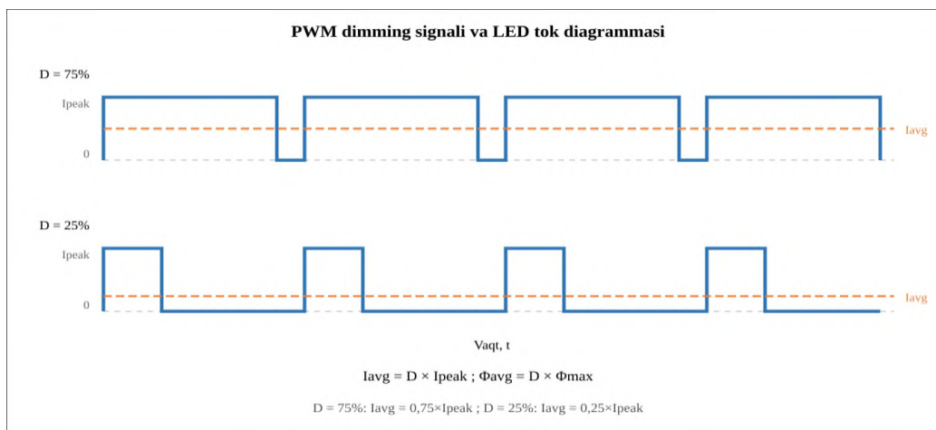
3-rasm. PWM dimming signali va LED tok diagrammasi ( D = 75\% va D = 25\% )
