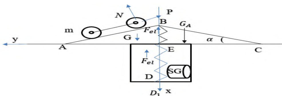
4-rasm. Qurilmaning hisob sxemasi
