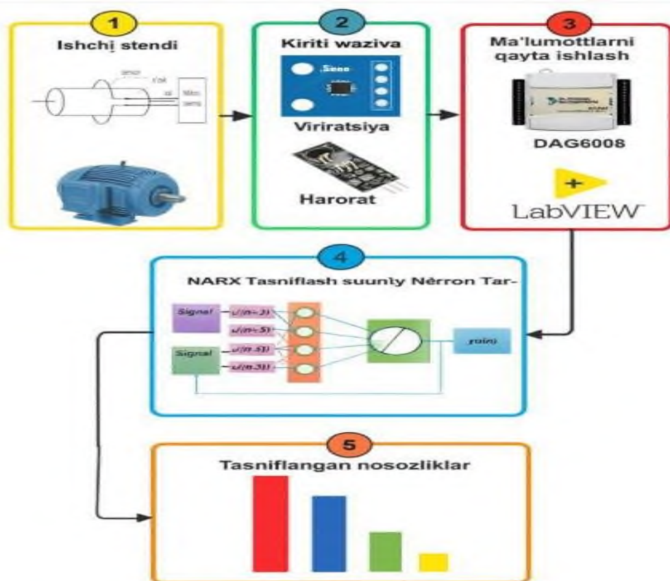
4-rasm. Jarayonning blok-sxemas.
