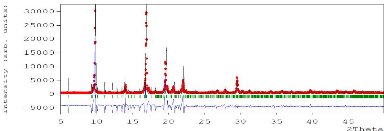
1-rasm. [\text{Co}(\text{tmphen})_3](\text{PF}_6)_2 kompleksining difraktogrammasi
